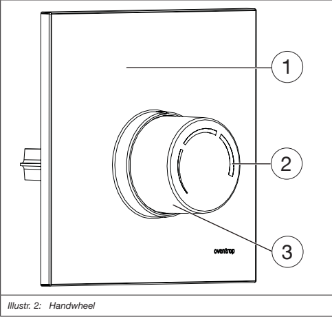
Illustr. 2: Handwheel
