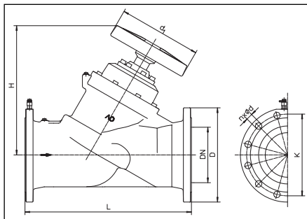
Illustr. 3 Dimensions DN 200 - DN 300
