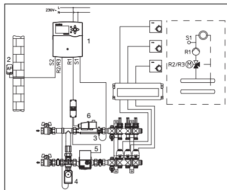
Illustr. 6.3 Connection summary of the components (one variable temperature circuit)
