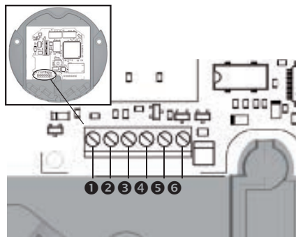
Connection terminals of the Datalog CS-BS-1
