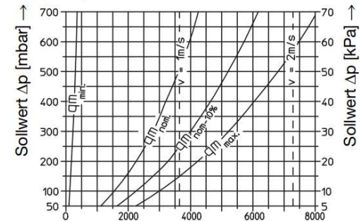
DN 32: kvs = 10,0
