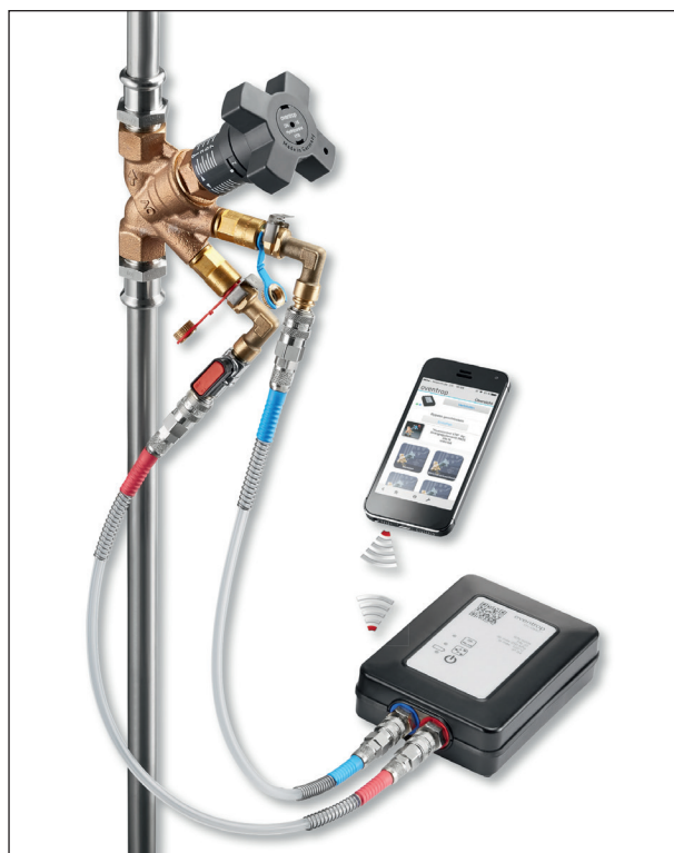
Measuring system “OV-DMC 3” item no. 1069278 with double regulating and commissioning valve “Hydrocontrol VTR”
