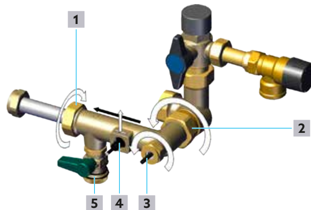
Abb. 5: Messturbine reinigen
