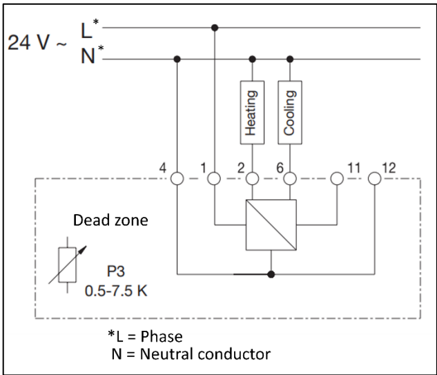
Wiring diagram
