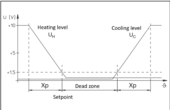
Function diagram
