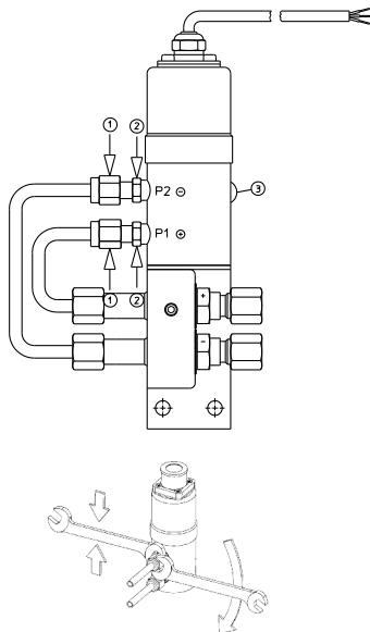
Illustr. 5: Deaeration
