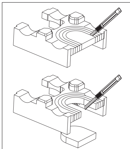
Illustr. 5.4 Insertion block with cutting for heat meter
