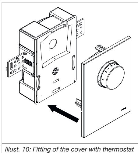
Illust. 10: Fitting of the cover with thermostat
