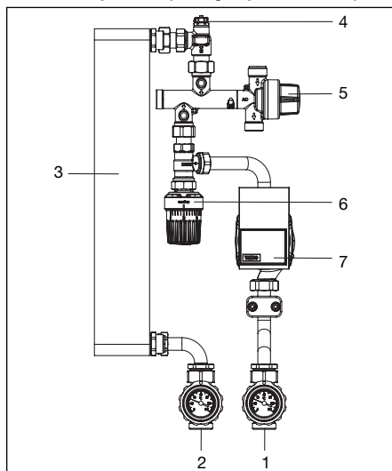
Illustr. 5.2: Primary circuit
