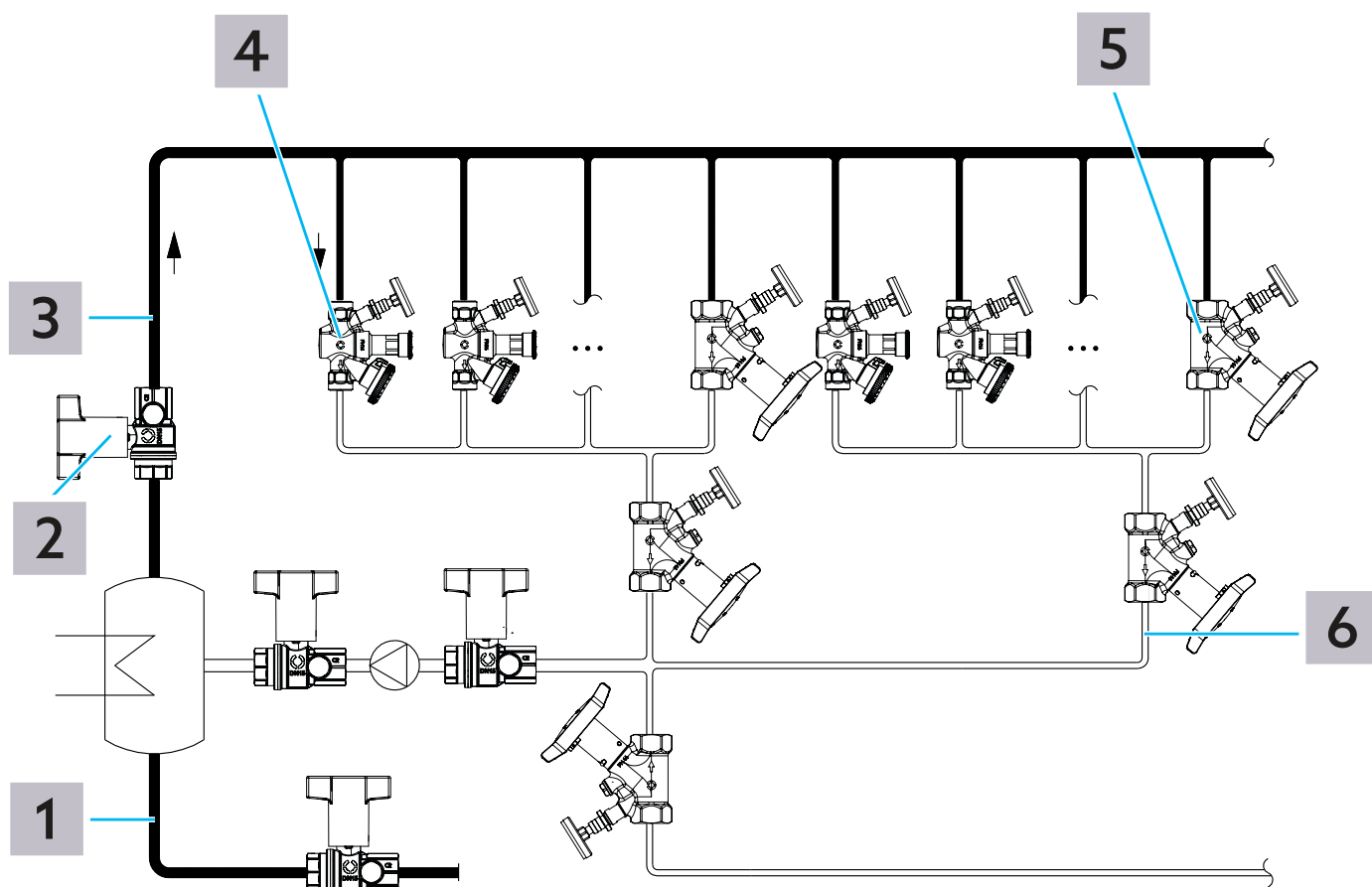
Fig. 4: System diagram
