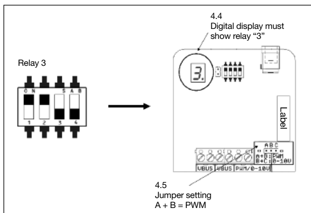
Illustr. 5.5 Relay addressing and jumper setting
