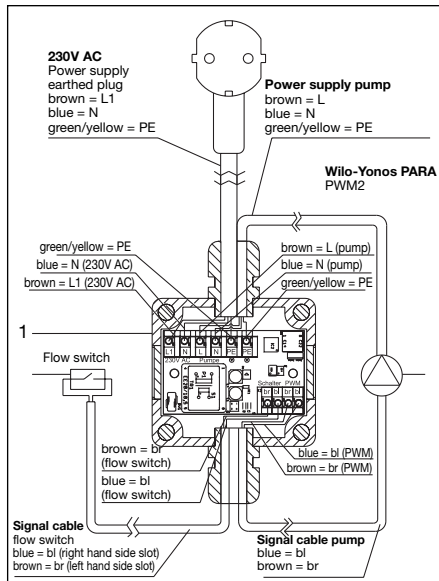
Illustr. 5.3: Cabling
