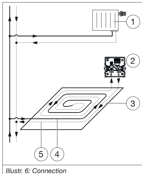
Illustr. 6: Connection
