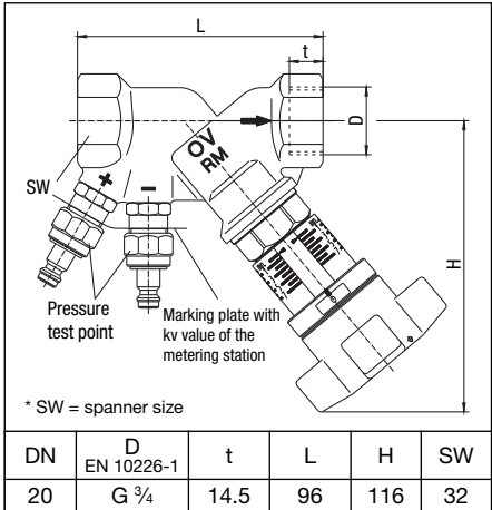
Illustr. 4.2 Dimensions “Hydrocontrol STR” with female thread
