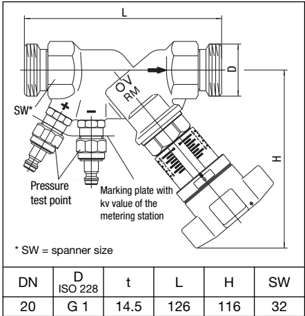
Illustr. 4.1 Dimensions “Hydrocontrol STR” with compression connection
