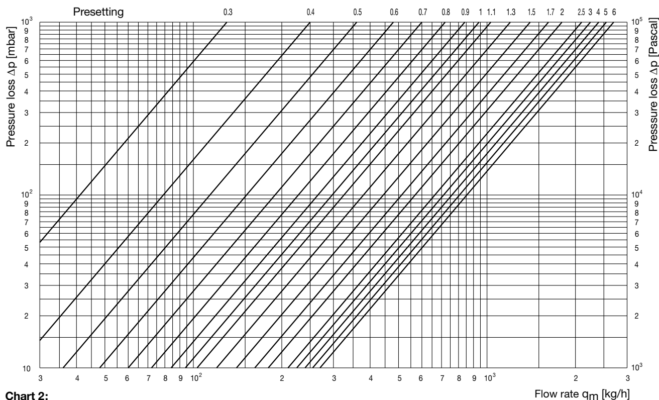
Chart 2: Pressure loss double regulating and commissioning valve "Hycococon VTZ" DN 20
