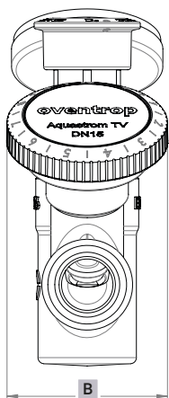
Fig. 3: Frontal dimensions
