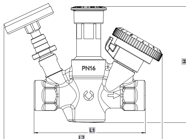
Fig. 2: Lateral dimensions
