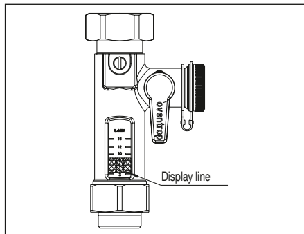
Illustr. 4.5 Balancing valve
