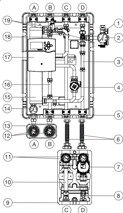
Illust. 2: Construction of the Regudis H-H
