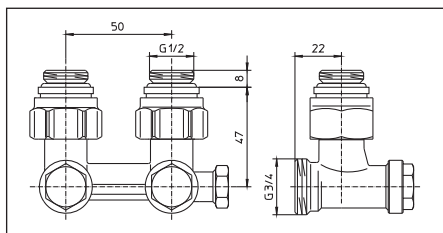
Abb. 6 Eckform, G 1/2 AG x G 3/4 AG
