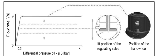
Illustr. 7 Flow characteristic line for different presetting
