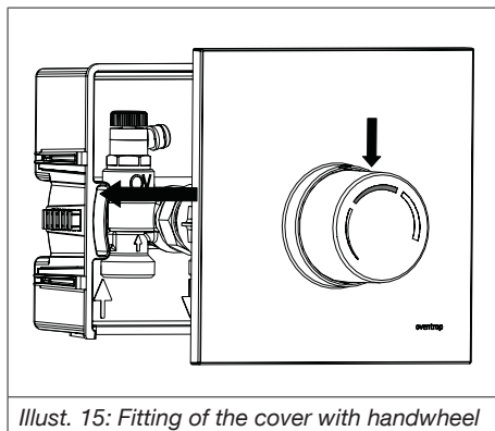
Illust. 15: Fitting of the cover with handwheel
