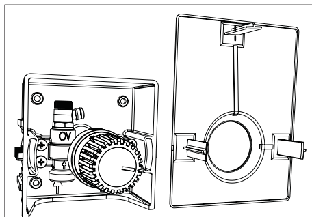
Illust. 18: Reverse side of the cover
