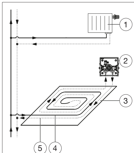
Illust. 10: Connection
