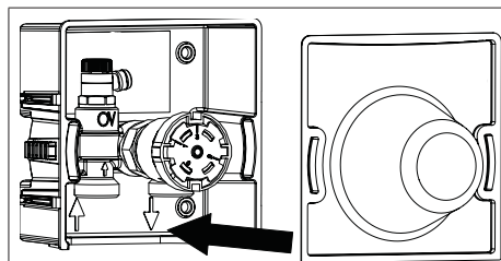
Illust. 12: Fitting of the protection cover
