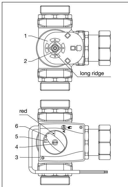
Illustr. 5.8 Installation 3-way mixing valve DN40 / DN50
