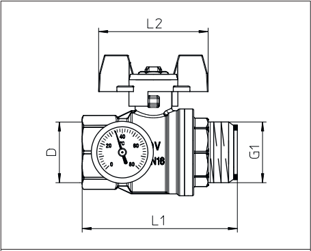
Abb. 5: Dimensions ball valve
