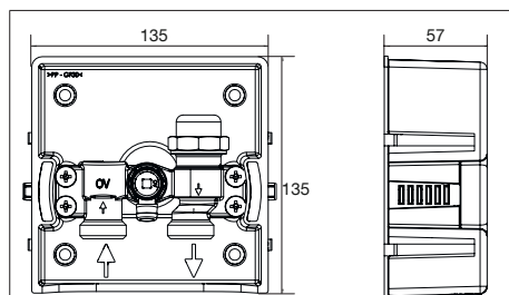
Illust. 3: Dimensions in mm
