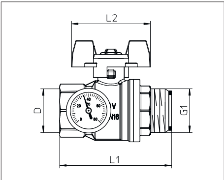
Illustr. 6: Dimensions of the ball valve
