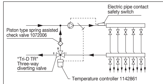
Installation example regulating set no. 3
