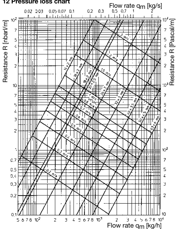
12 Pressure loss chart
