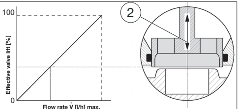
Fig. 5: Linear characteristic line of the regulating unit
