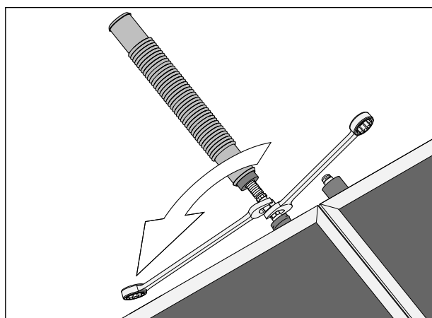
Illustr. 4 Tighten connection with 1/4 turn. Hold firm while tightening to avoid damage to the collector and coupling hose. !
