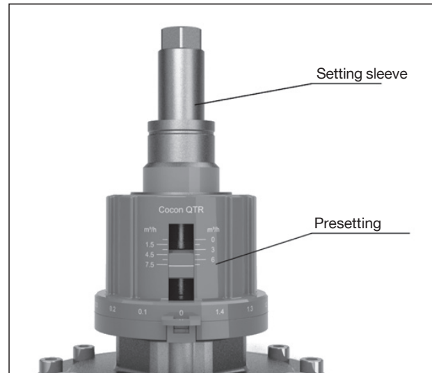
Setting sleeve
