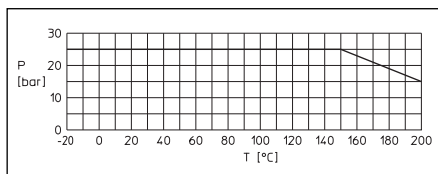
Illustr. 4.3 Max. working pressure p_s depending on the working temperature t_s
