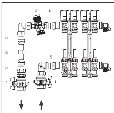
Illustr. 4: Heat meter connection set, angle pattern, extent of supply and location of the components for left hand side connection
