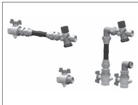
Illustr. 1 Heat meter connection set, straight and angle pattern
