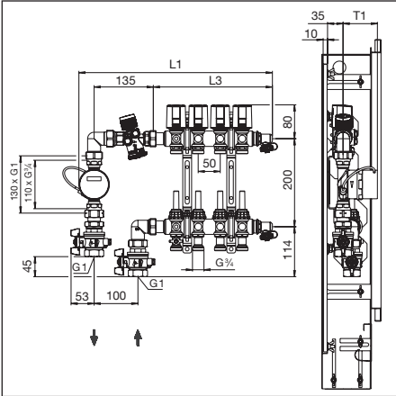
Illustr. 2 Example: Heat meter connection set, angle pattern and stainless steel distributor/collector "Multidis SF" for surface heating systems, length and depth
