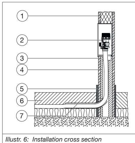
Illustr. 6: Installation cross section
