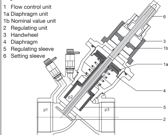
Pressure independent control valve “Cocon QTR”
