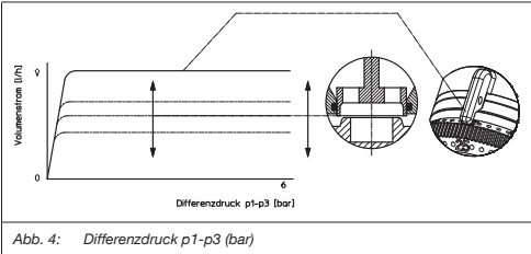
Abb. 4: Differenzdruck p1-p3 (bar)
