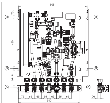
Illustr. 6.2 Connection scheme ball valve connector block
