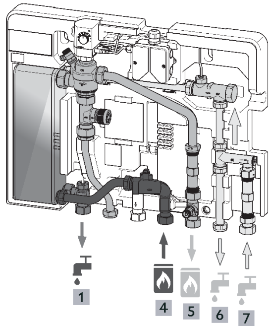
Warm tapwater
