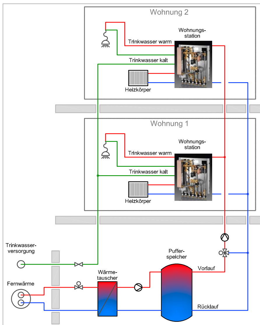
Installation scheme for the new "Regudis" dwelling station: a boon for comfort and hygiene
