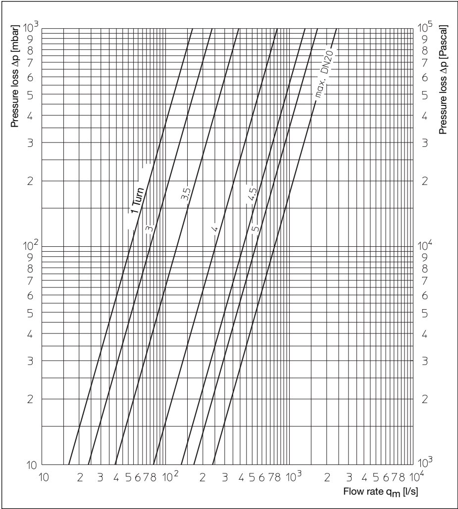
Illustr. 9.1: Chart regulating insert for different presettings
