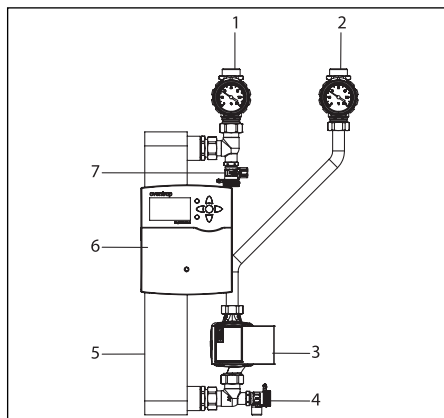
Illustr. 6: Primary circuit
