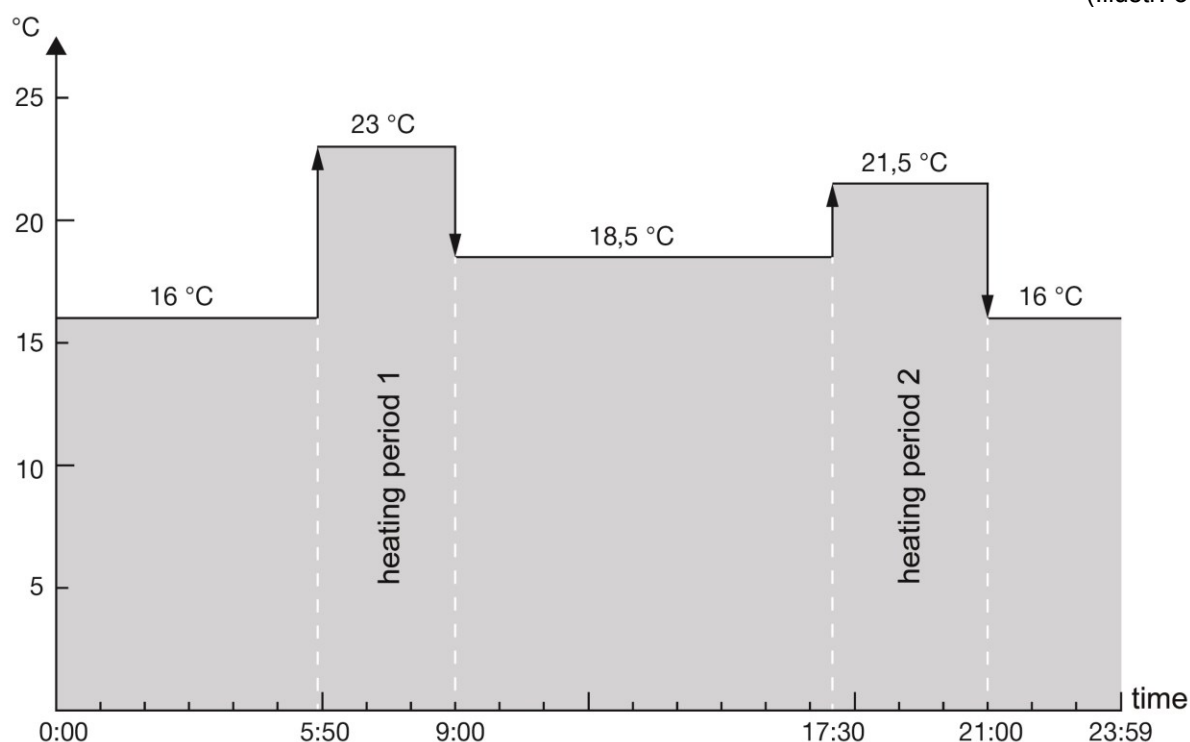
24 hour view of the heating/setback periods programmed in the above example
