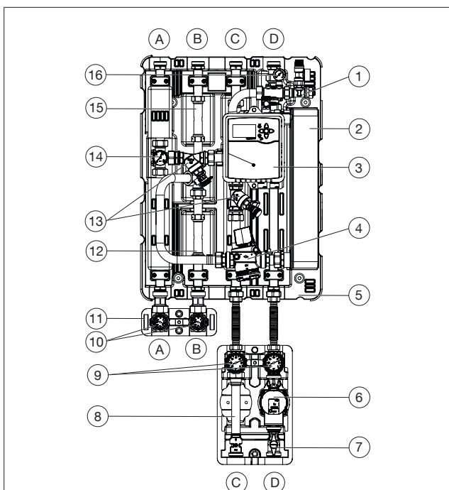
Illust. 2: Construction of the Regudis H-M
