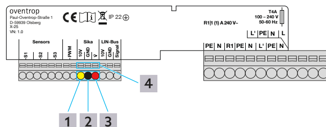
Fig. 9: Plaque à bornes Regumag X-25
