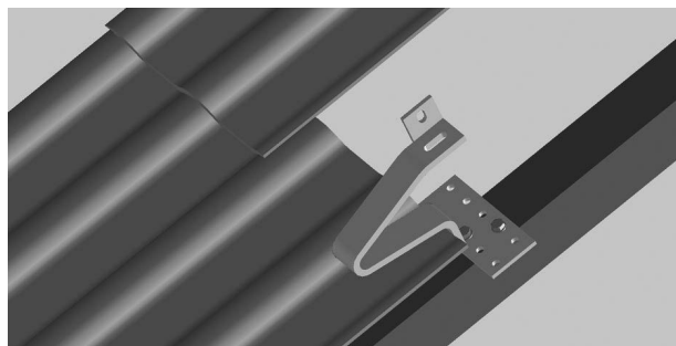
Illustr. 6: Fitting of roof hooks (Illustr. roof hook item no. 1361262)
