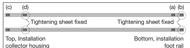
Illustr. 5: Pre-assembled mounting rail set for roof installation, tightening sheets (b) and (d) are fixed
