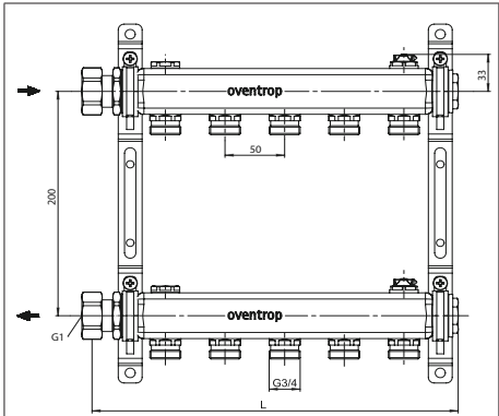
Illustr. 2: Dimensions in mm (front view)
