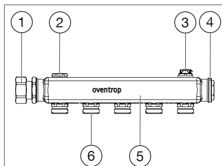
Illustr. 1: Construction
