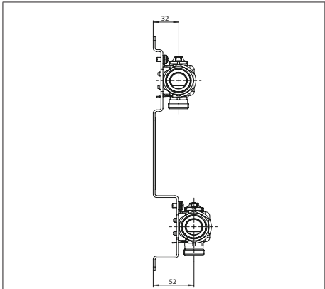
Illustr. 3: Dimensions in mm (side view)
