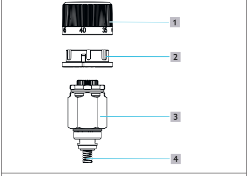
Illustr. 1: Construction
