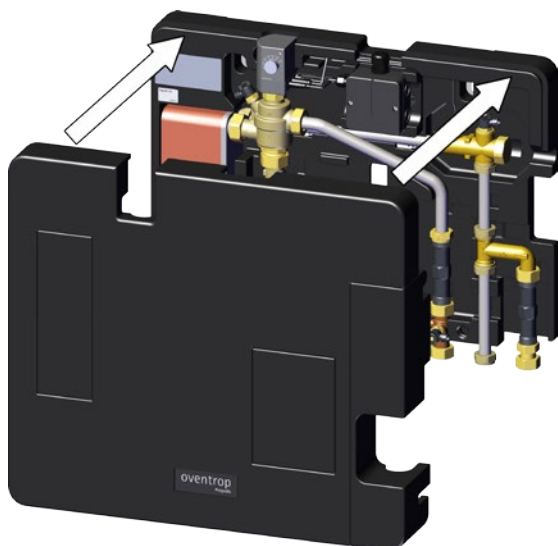
Fig. 2: Mounting the upper thermal insulation shell
